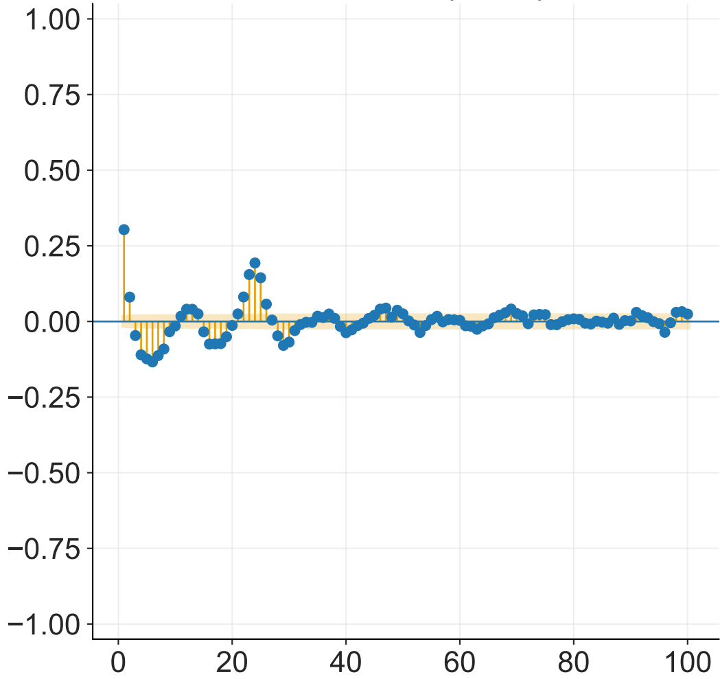
ACF MSM (2020)
